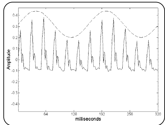
Example of an Enveloped Time Waveform (Inner Race).
