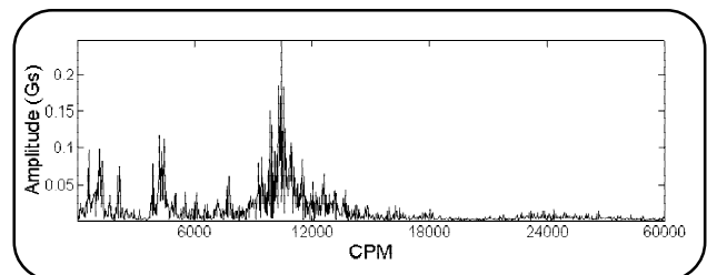
A Spalled Bearing's Acceleration Vibration Spectrum.
