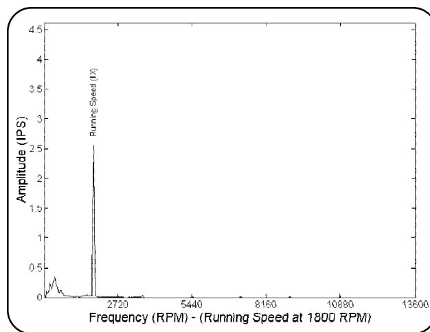
A FFT Spectrum Showing Imbalance.
